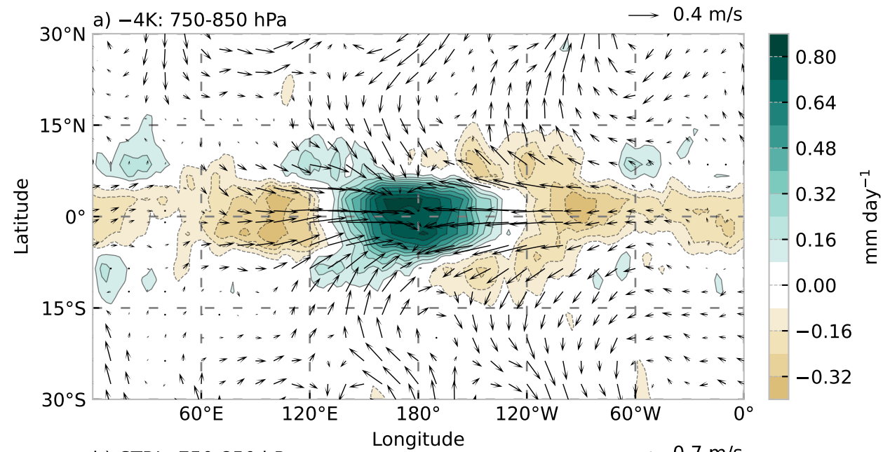
Precipitation and Lower Level Winds
