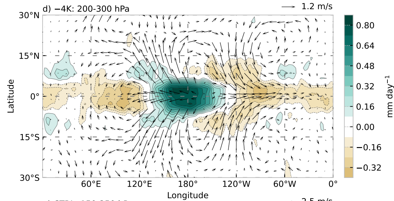
Precipitation and Upper Level Winds
